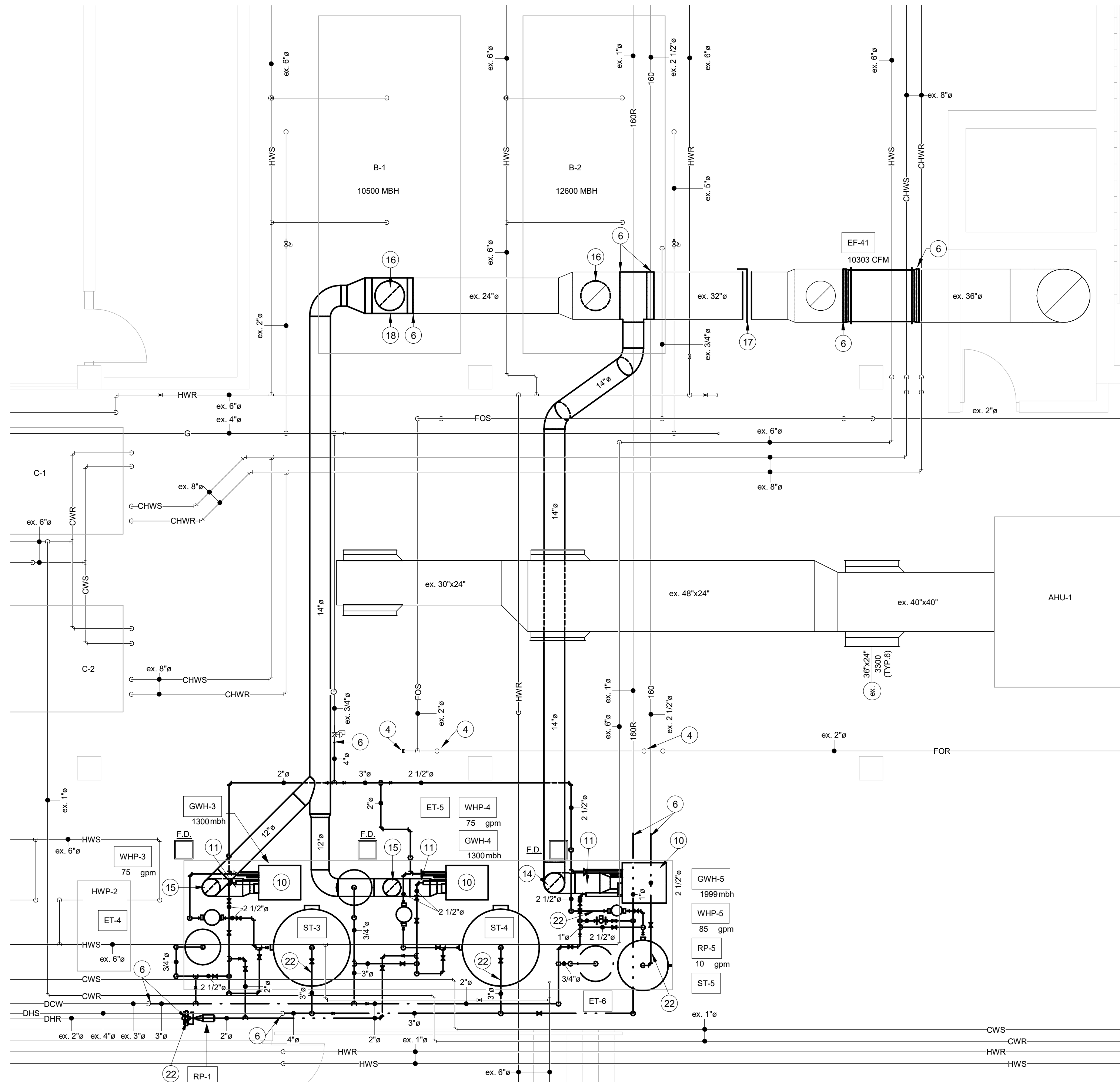
1 South Mech Plan 1/4" = 1'-0"
