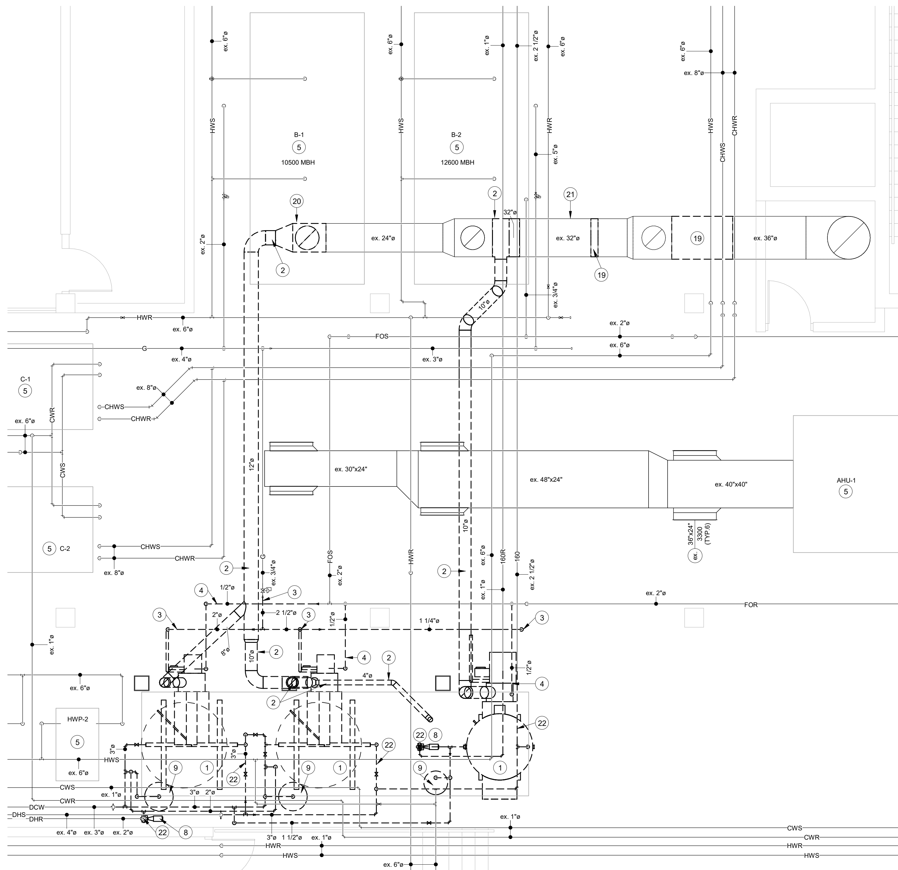
2 South Mech Demo Plan 1/4" = 1'-0"
