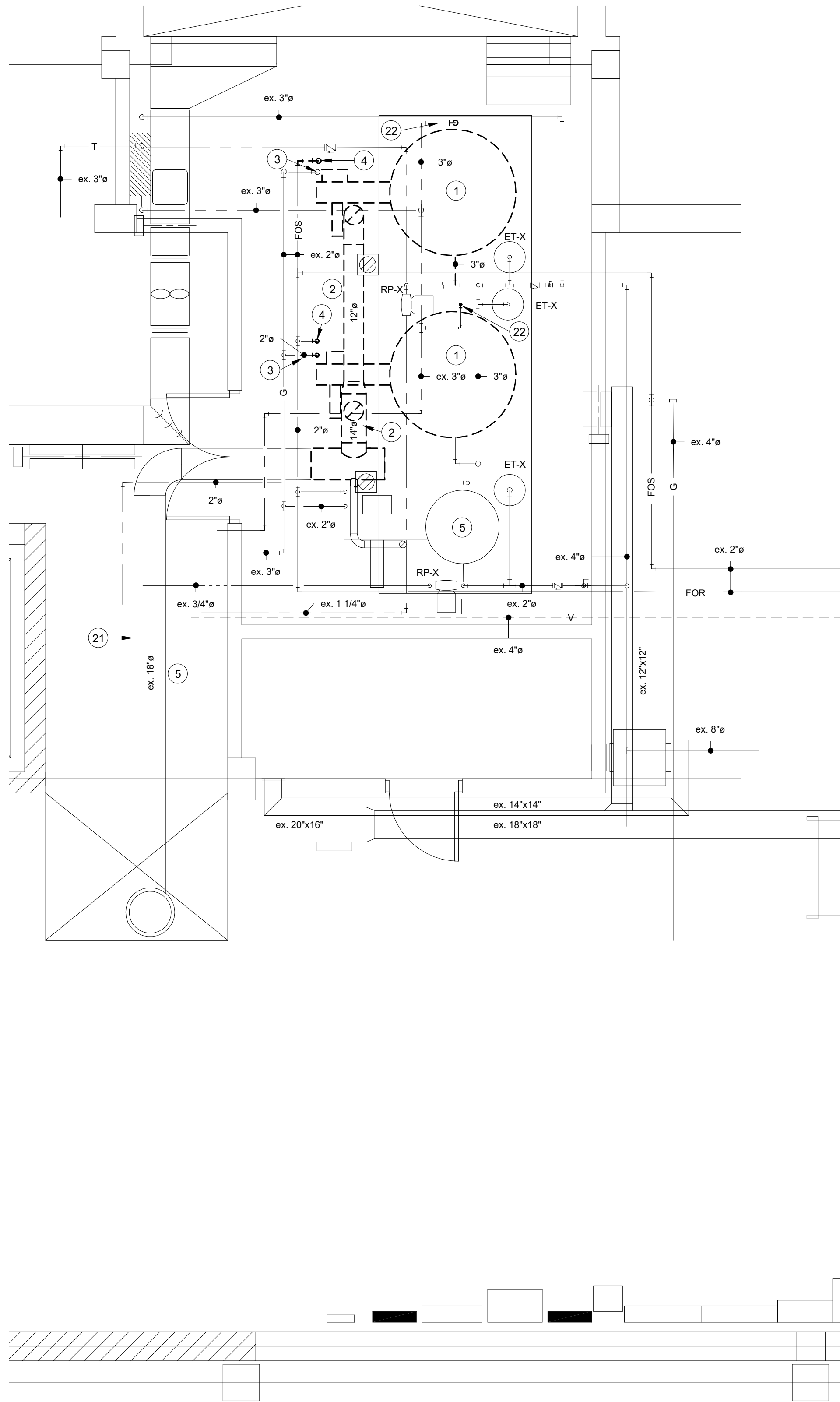
② North Mech Demo Plan 1/4" = 1'-0"
