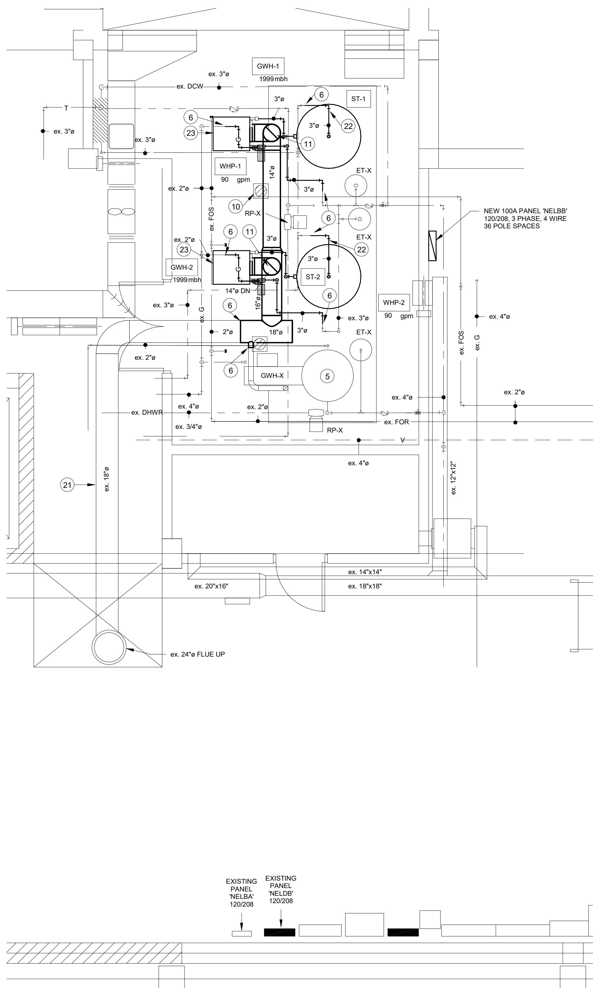
① North Mech Plan 1/4" = 1'-0"
